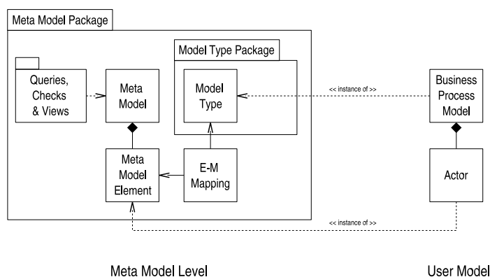
Fig. 1. The notions on meta model level and user model.
